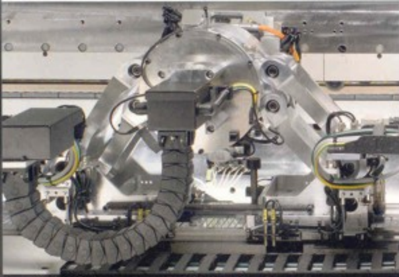
NOVIMAT Performance: neues Kopierfräsaggregat
